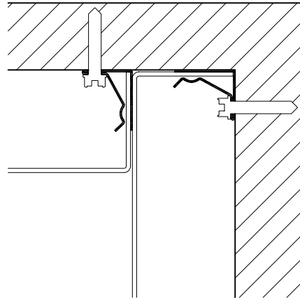
STANDARD INSIDE CORNER
