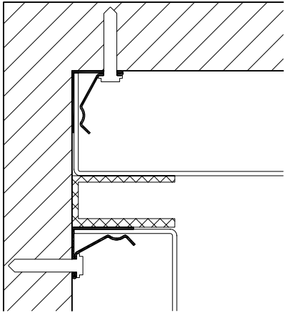
INSIDE CORNER OPEN REVEAL
