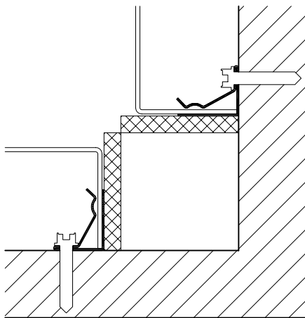
INSIDE CORNER DOUBLE REVEAL
